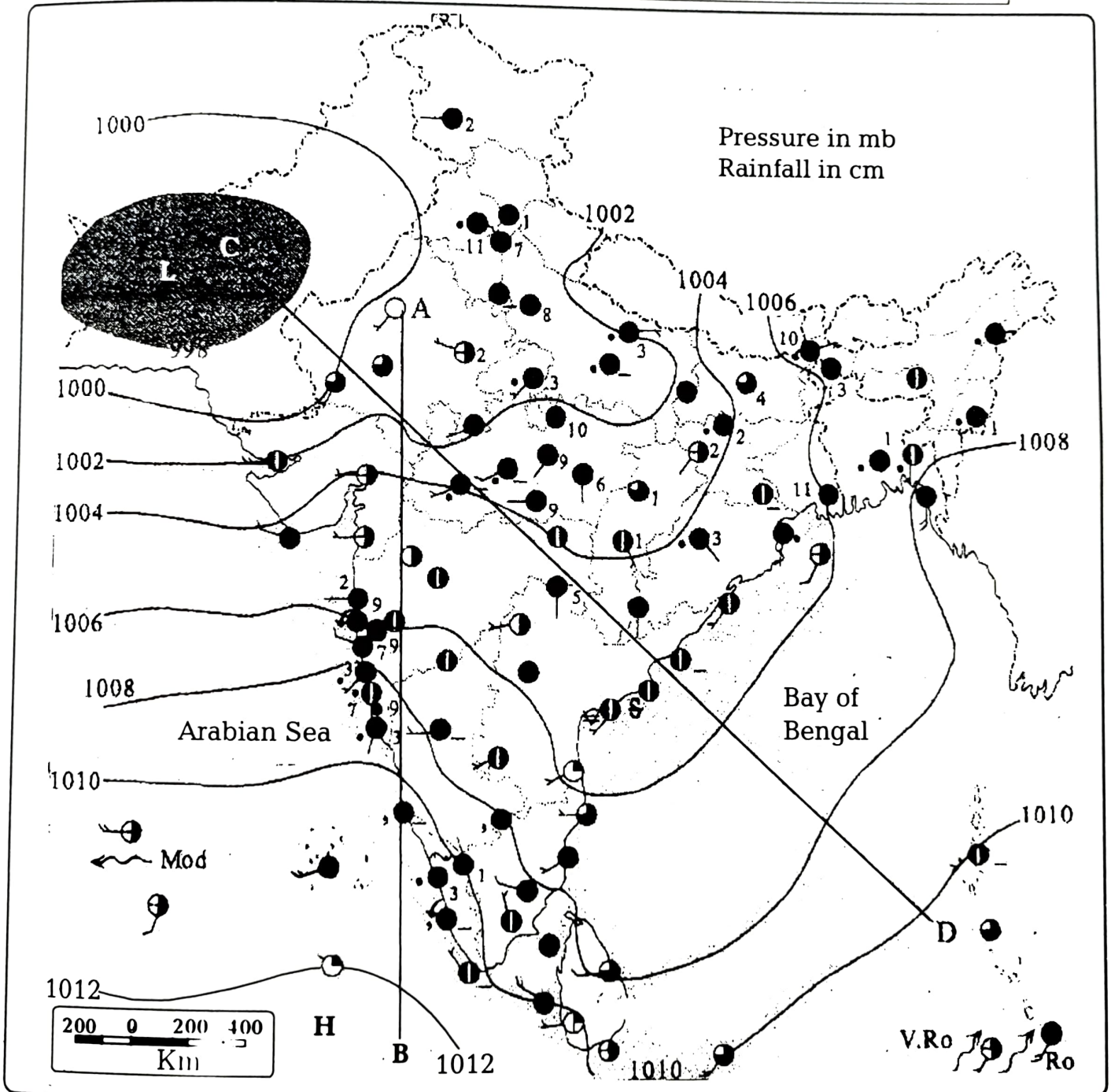
Fig. 3.16: Indian Daily Weather Report (Map No. 2)
